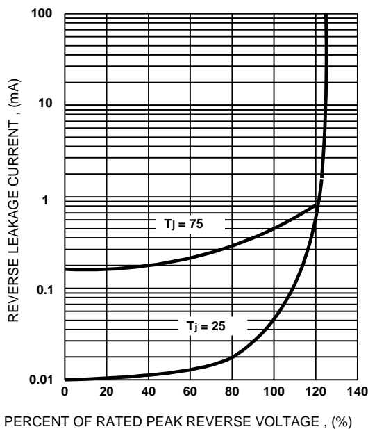
Figure 5. Typical Reverse Characteristics
