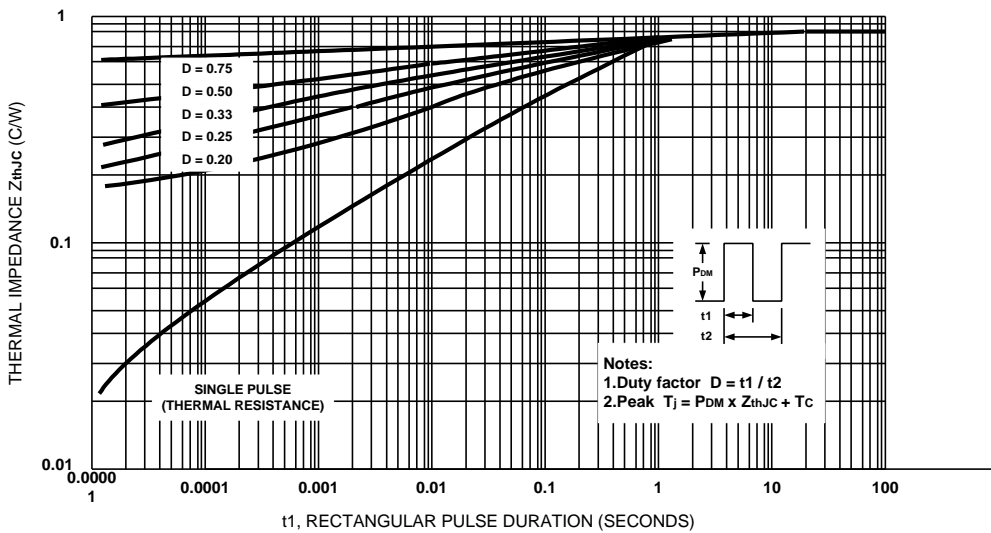
Figure 4. Max. Thermal Impedance Z_{thJC} Characteristics (PerLeg)
