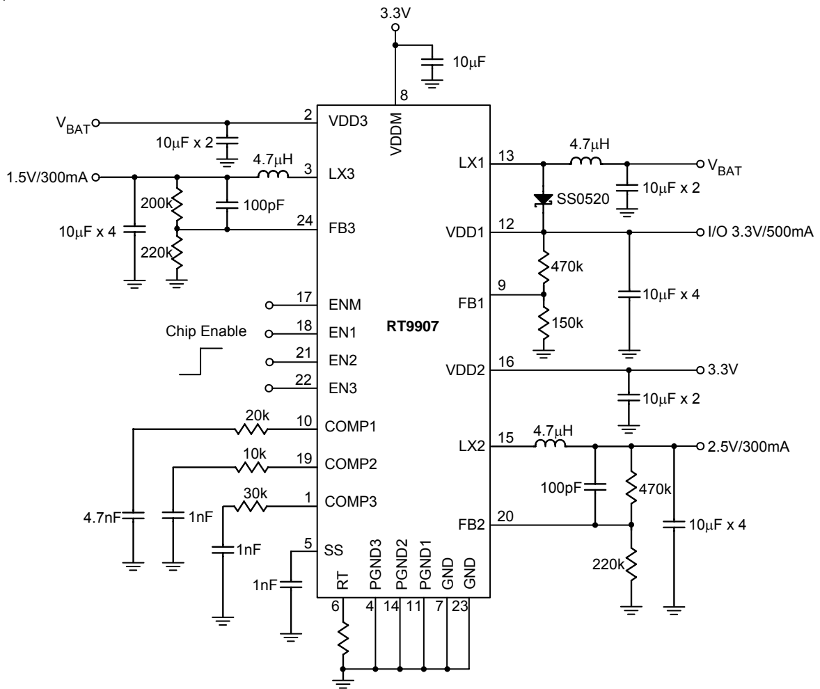
Figure 2. Typical Application Circuit for 2-AA Battery Supply
