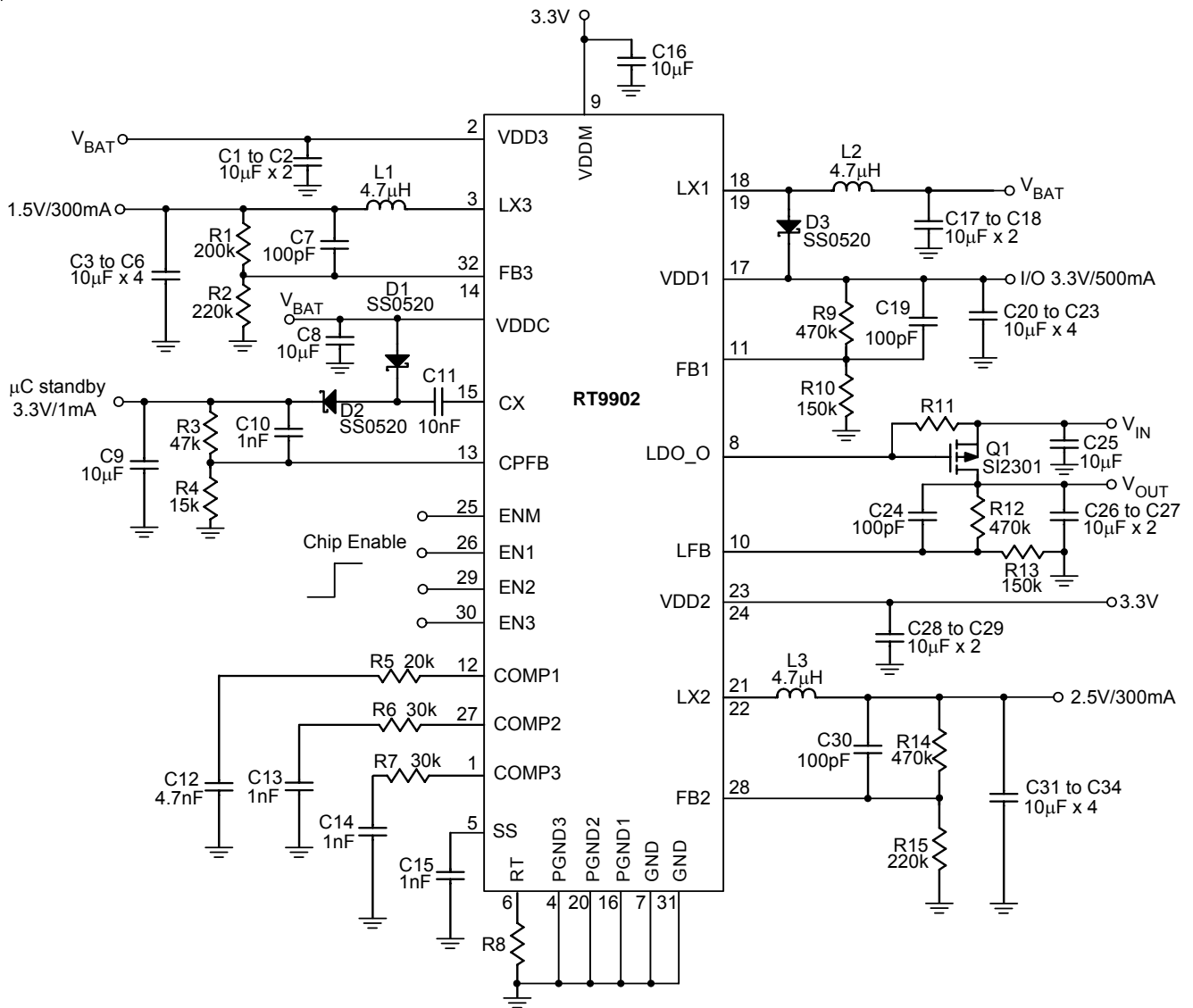
Figure 3. Typical Application Circuit from 2-AA Battery Supply
