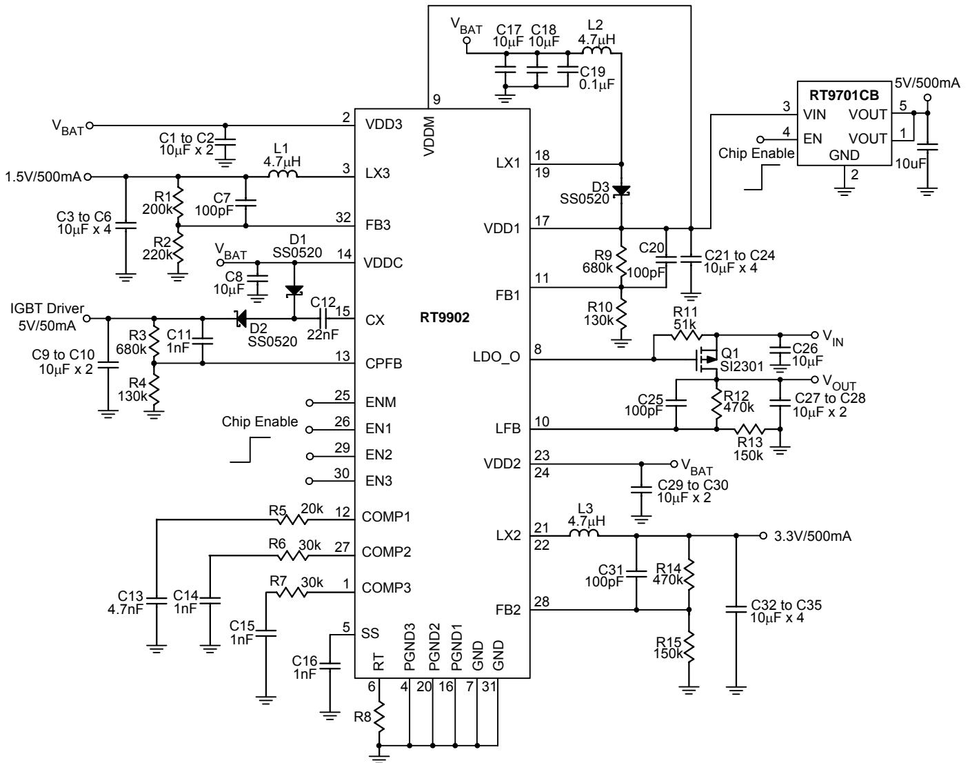
Figure 2. Typical Application Circuit from 1-cell Li+ Battery
