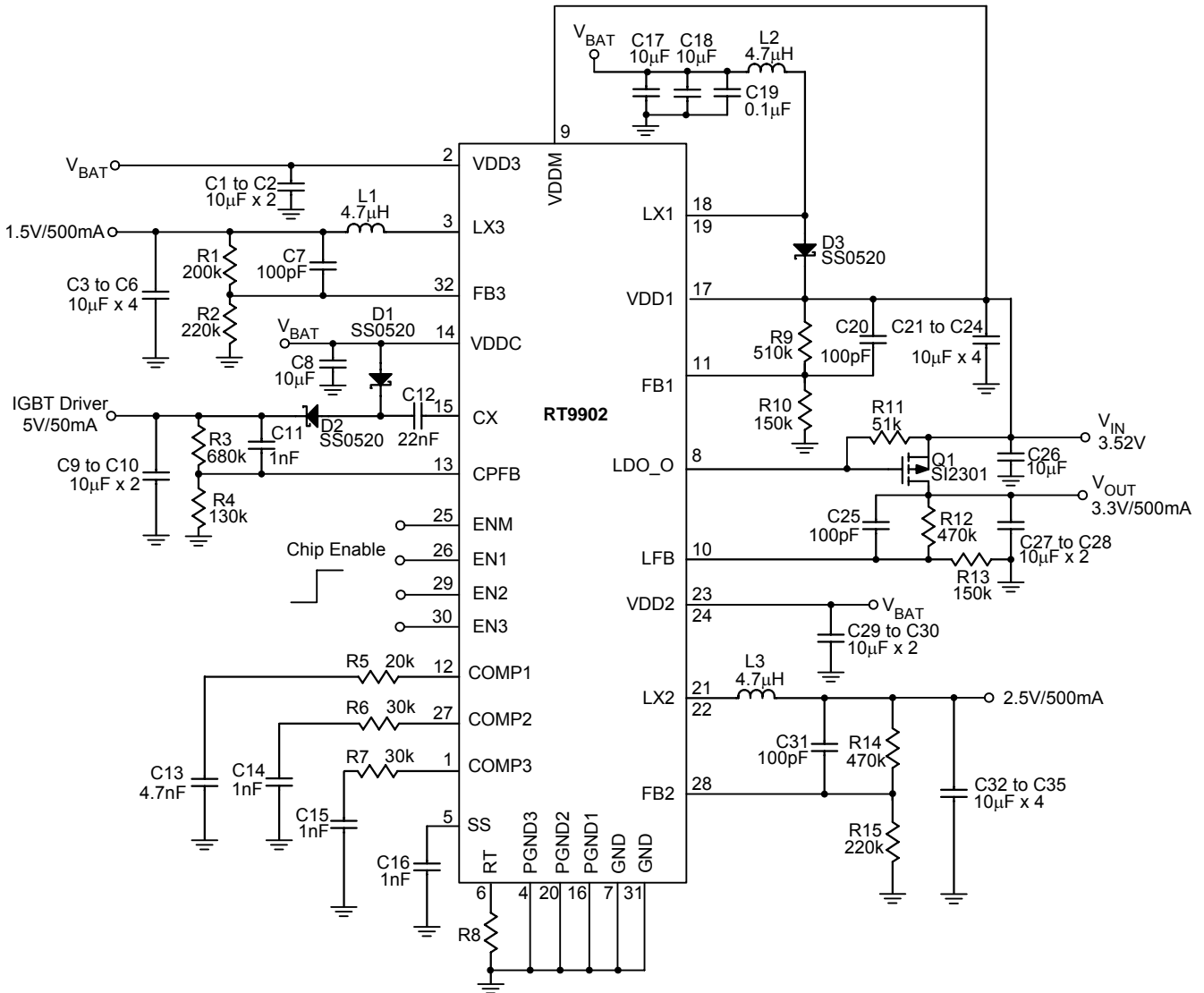
Figure 1. Typical Application Circuit from 1-cell Li+ Battery
