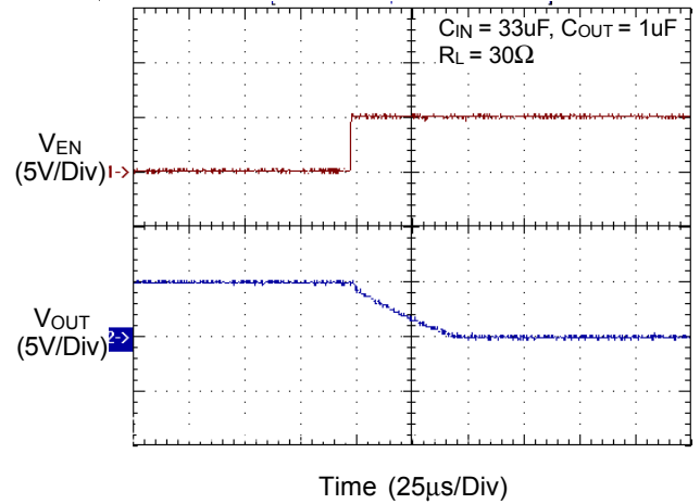
Turn-Off Response
