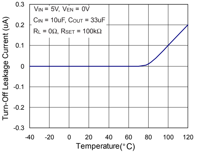
② Turn-Off Leakage Current vs. Temperature
