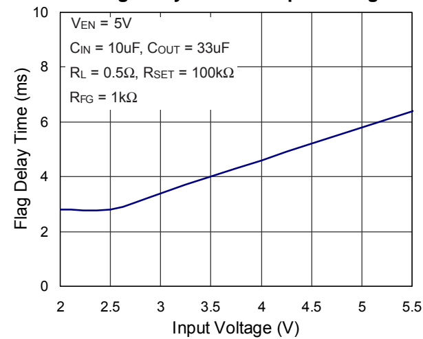
④ Flag Delay Time vs. Input Voltage
