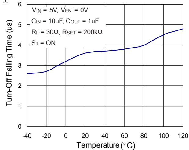
① Turn-Off Falling Time vs. Temperature
