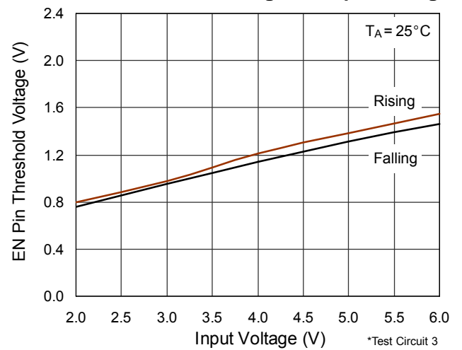
EN Pin Threshold Voltage vs. Input Voltage
