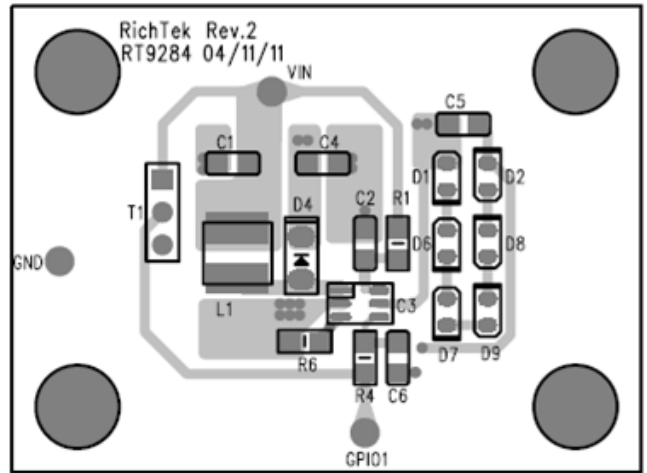
Figure 8. Top Layer
