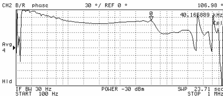
Figure 29. The Frequency Response with No Load
