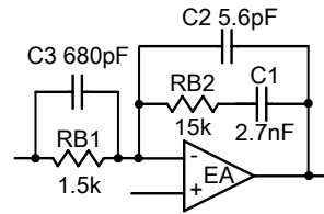
Figure 28. Type 3 compensation network of EA
