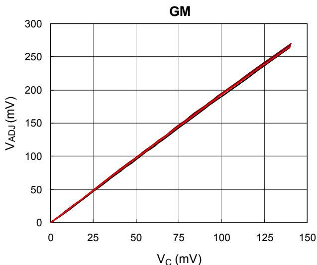
Figure 4. The Linearity of GMx
