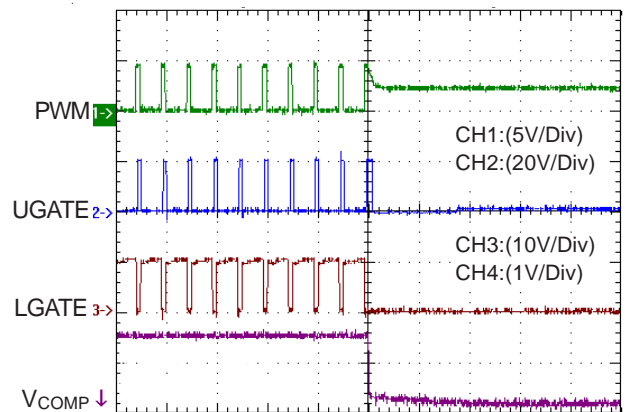
Power-Off @ I<sub>OUT</sub> = 60A
