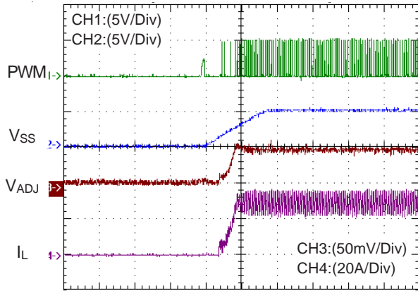
Relationship Between Inductor Current and V<sub>ADJ</sub>
