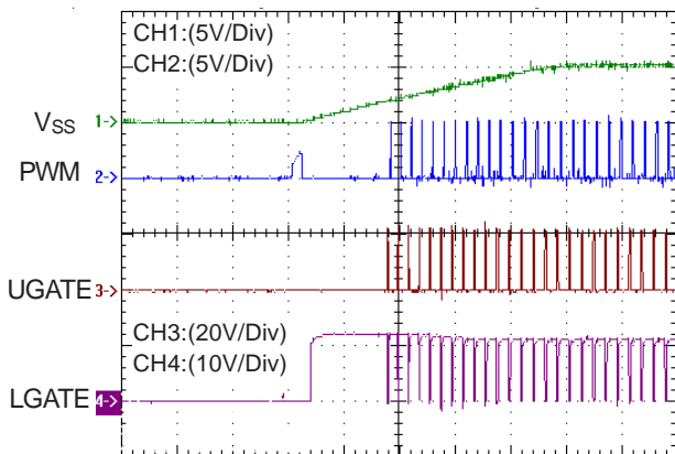
Power-On @ I<sub>OUT</sub> = 60A
