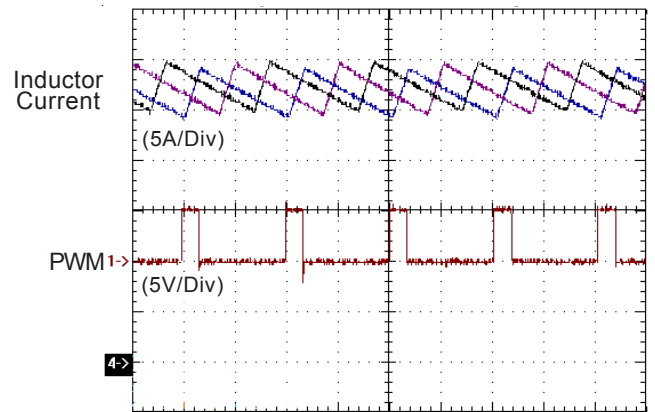
Time (2.5μs/Div)
