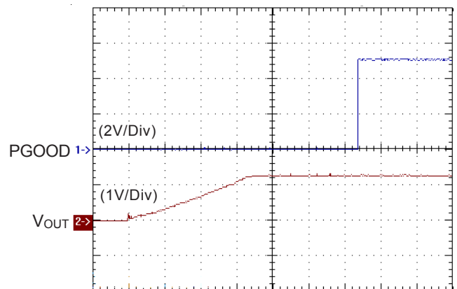
Time (5ms/Div)
