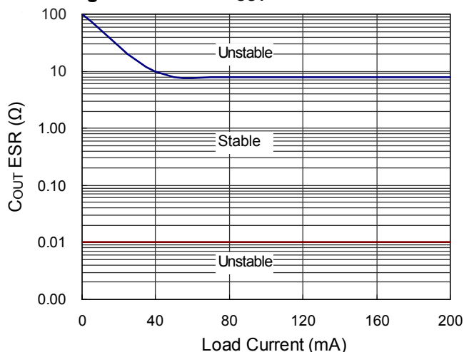
Region of Stable C_{\text{OUT}} ESR vs. Load Current
