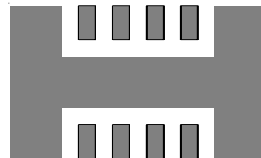
Figure 10 (d). Copper Area = 50mm 2 , θ JA = 51°C/W
