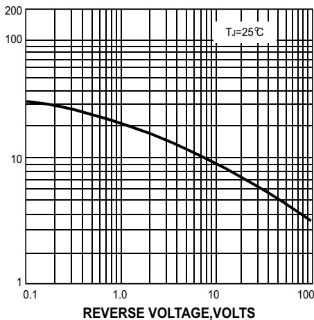
FIG. 5-TYPICAL JUNCTION CAPACITANCE
