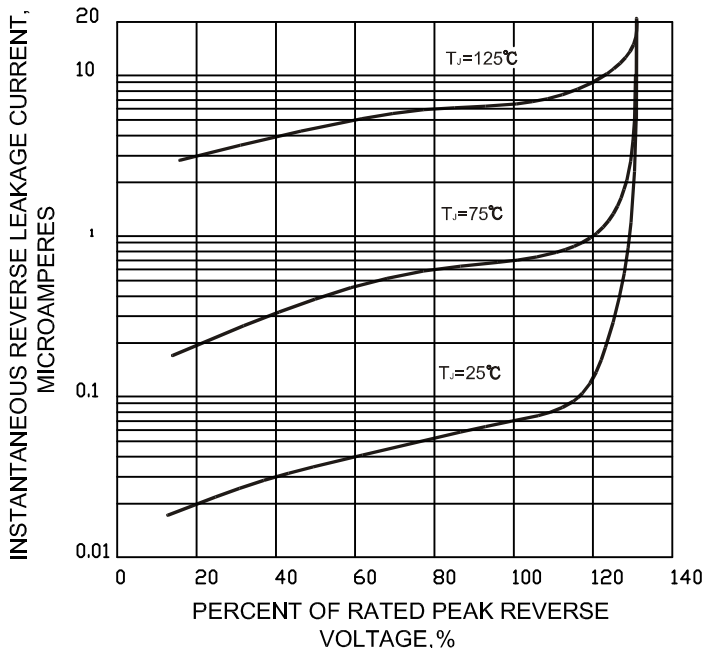
FIG.4-TYPICAL REVERSE CHARACTERISTICS
