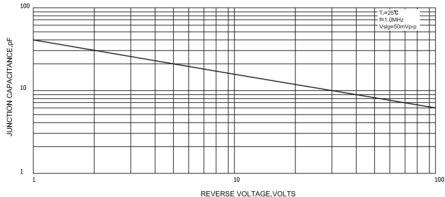
FIG.5-TYPICAL JUNCTION CAPACITANCE
