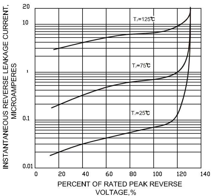
FIG.4-TYPICAL REVERSE CHARACTERISTICS
