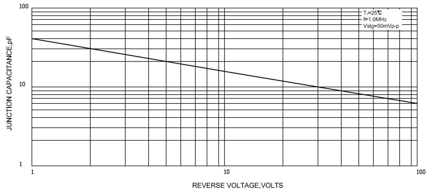
FIG.5-TYPICAL JUNCTION CAPACITANCE
