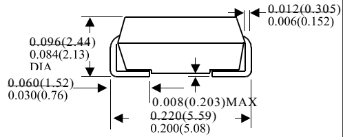
Dimensions in inches and (millimeters)
