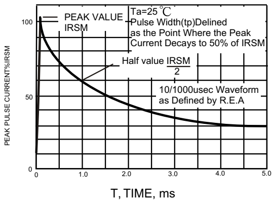
FIG.5-PULSE WAVEFORM
